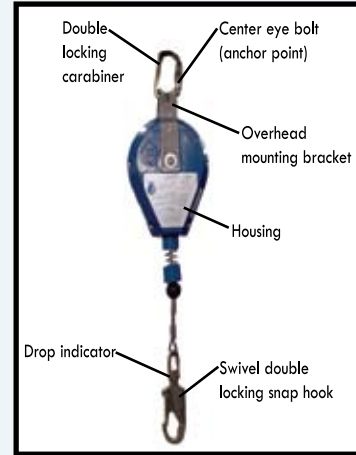
FS 2007 LIGHTWEIGHT & COMPACT 7 FT. WEB RETRACTABLE
